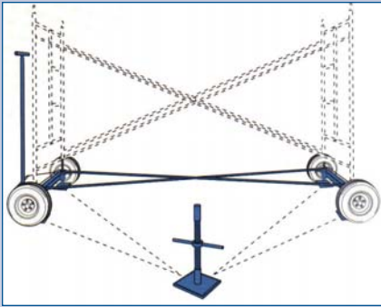
G Scaffold Wagon
