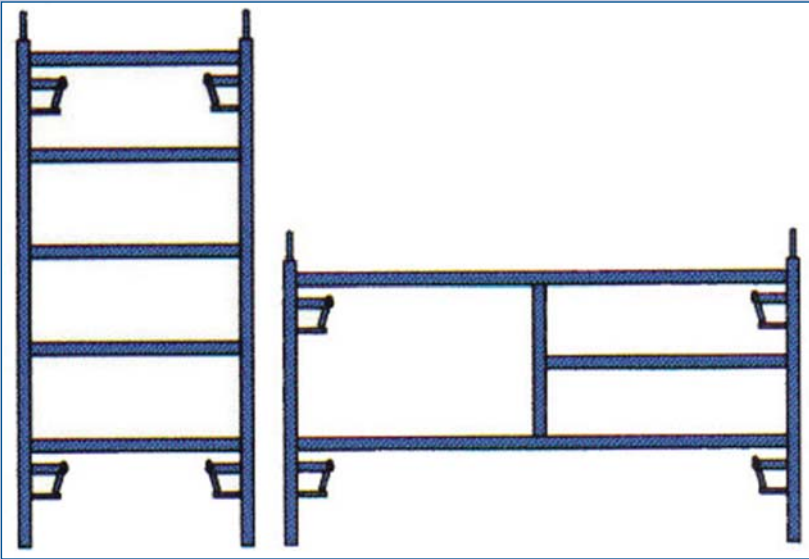
A Frame - 5' X 3'
